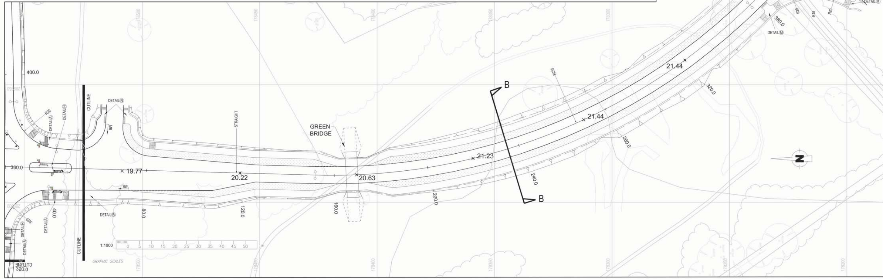
GENERAL ARRANGEMENT - INTERNAL ROAD: NORTHERN SECTION SCALE 1:1000
